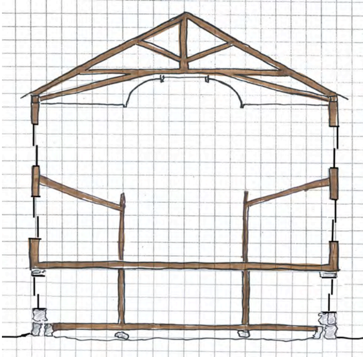
Sketch of timber frame 1811 as built with ceiling recessed cove, side balconies, short windows and full height finished basement.
